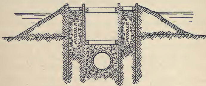
FIG. 31.—COFFER-DAM PUDDLE-WALLS.
